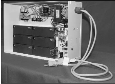
DIMENSIONS: 17.5" W X 10.8" H X 5.0" D
