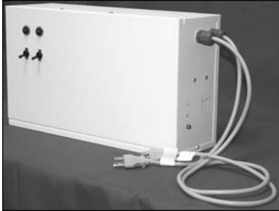
DIMENSIONS: 17.5" W X 10.8" H X 5.0" D
