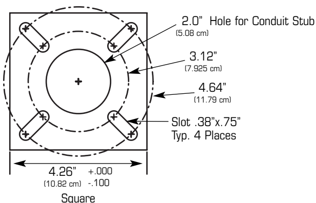
Base Details
